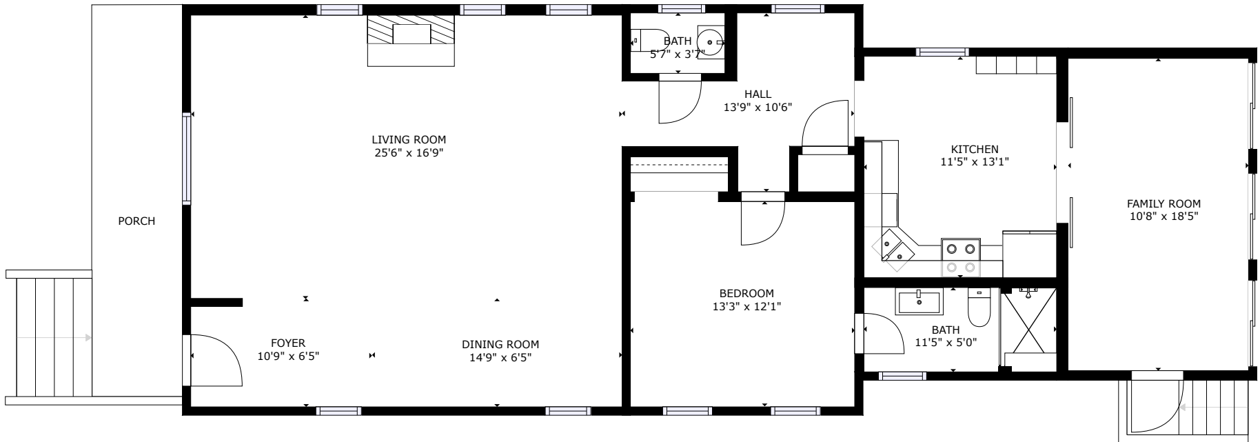
FLOOR 1
