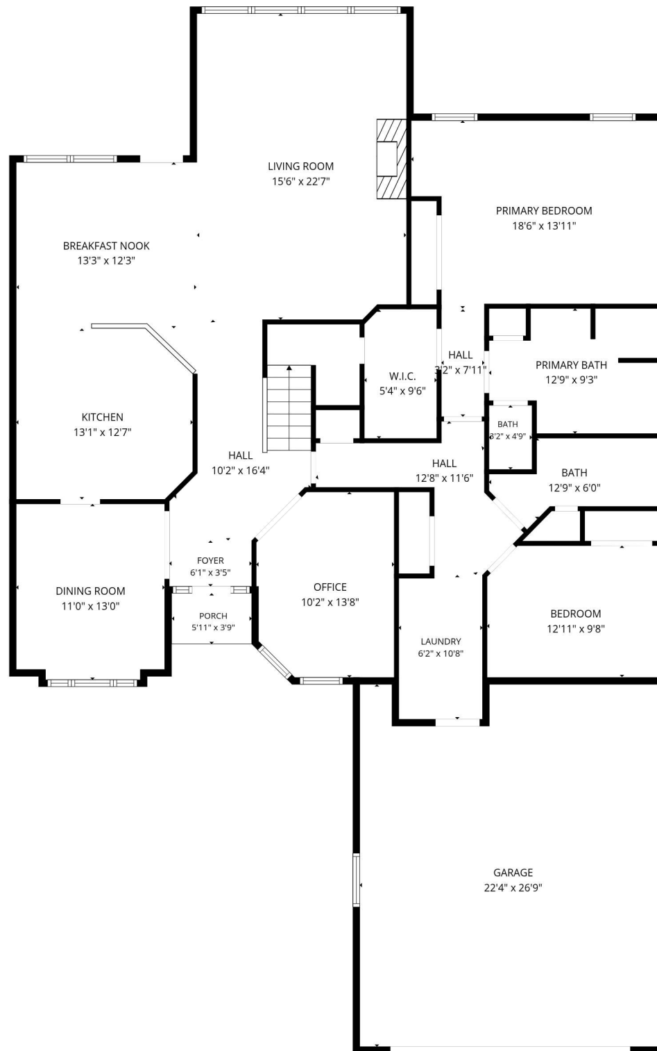
1st floor
