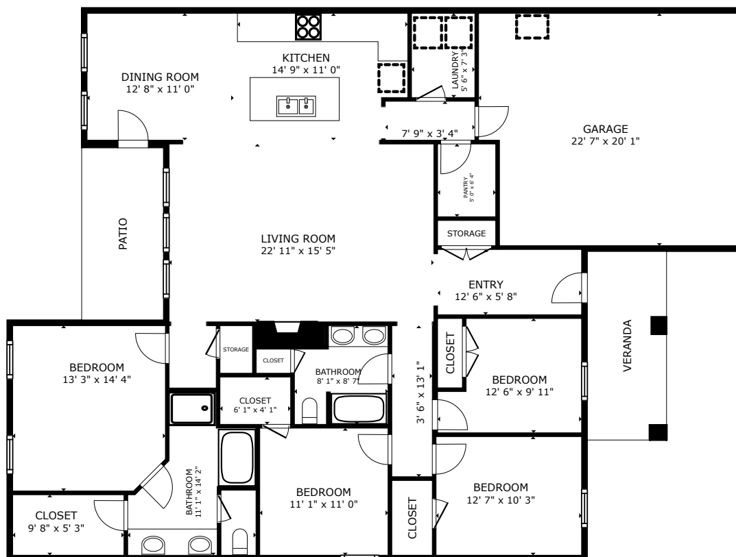
FLOOR PLAN
