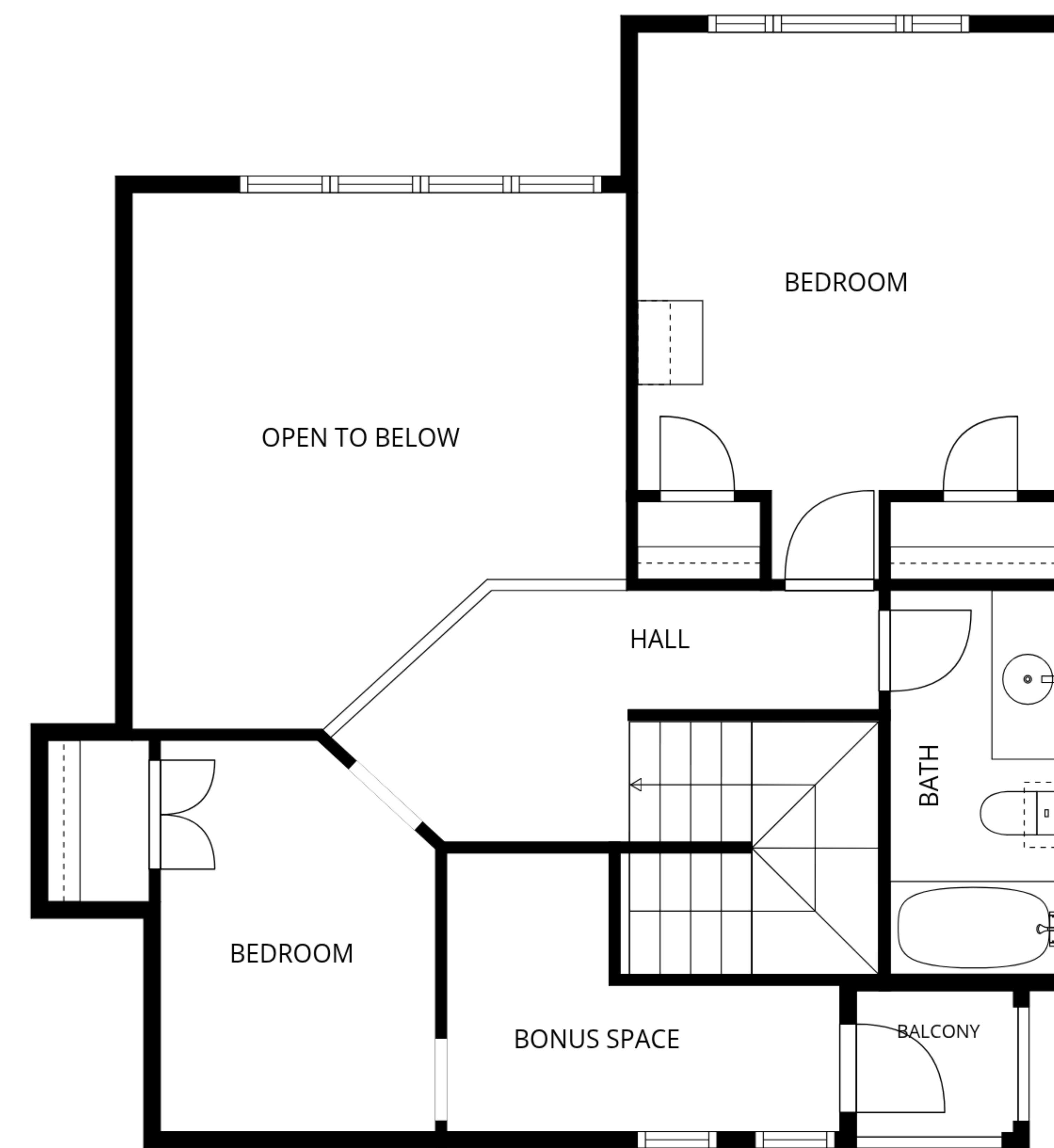
2nd floor
