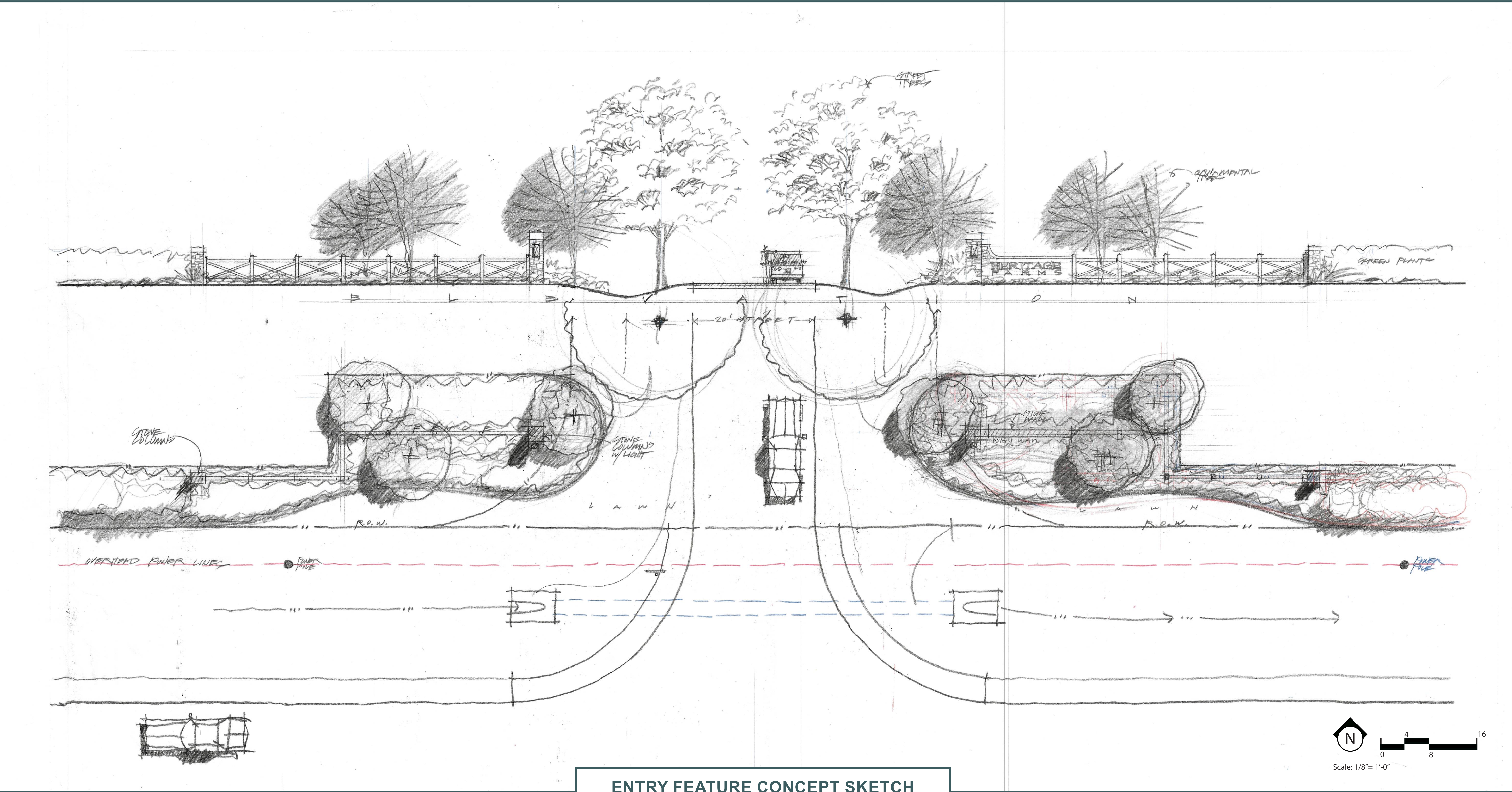
ENTRY FEATURE CONCEPT SKETCH SCALE: 1/8" = 1'-0"
