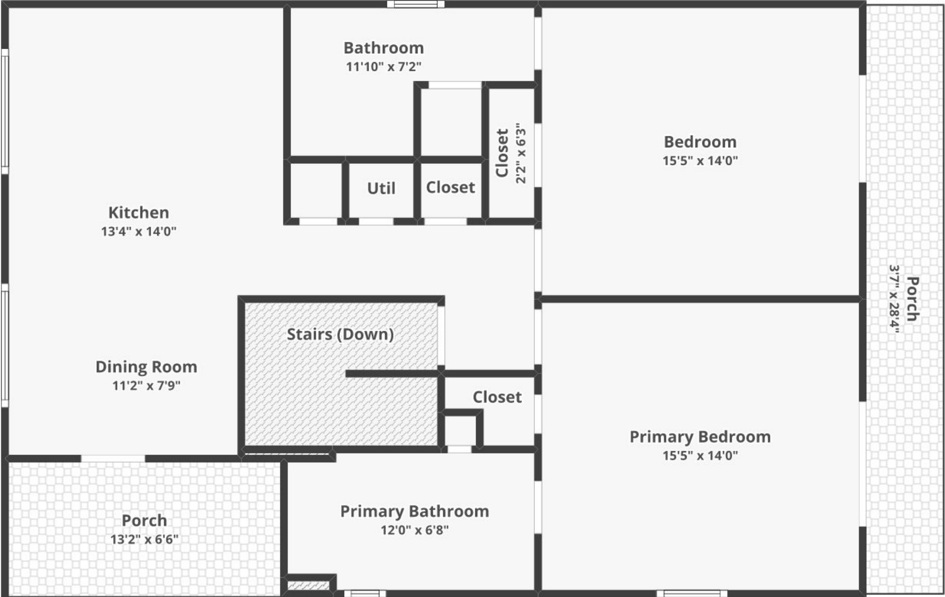
FLOOR 3
