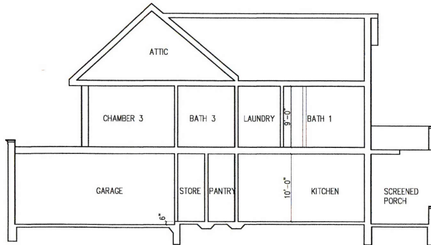
BUILDING (A-A) SECTION SCALE: 1/4"=1'-0"
