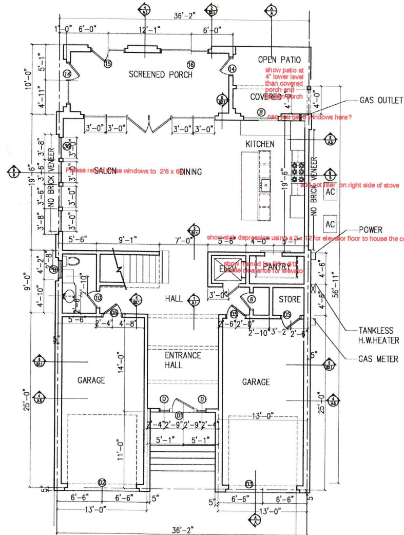
1 1ST FLOOR PLAN VIEW SCALE: 1/4"=1'-0"
