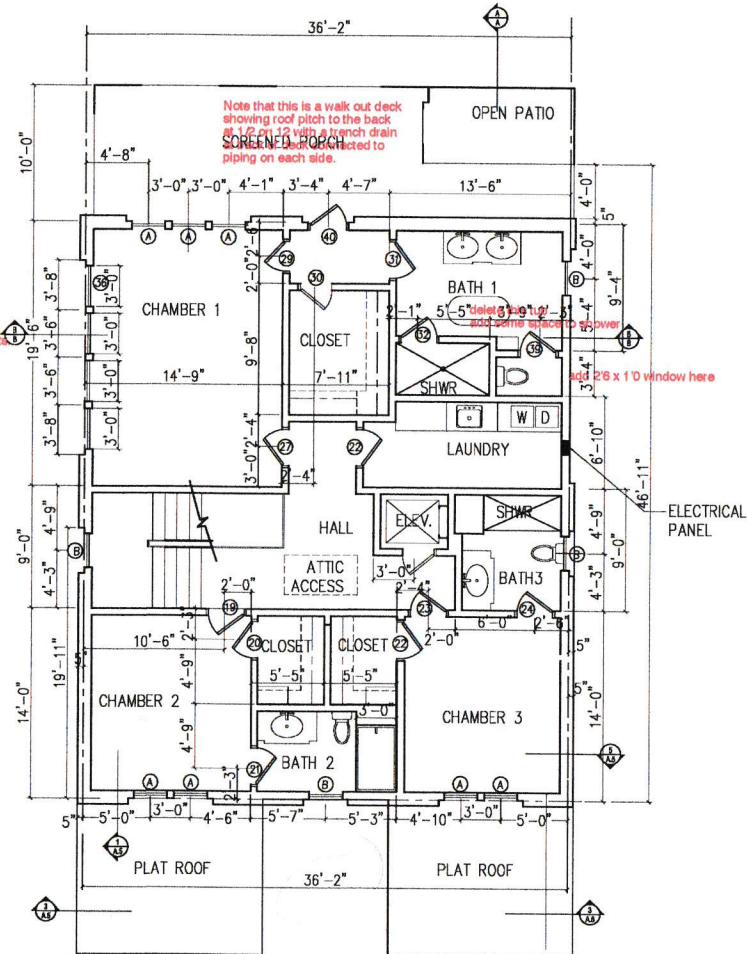
2 2ND FLOOR PLAN VIEW SCALE: 1/4"=1'-0"
