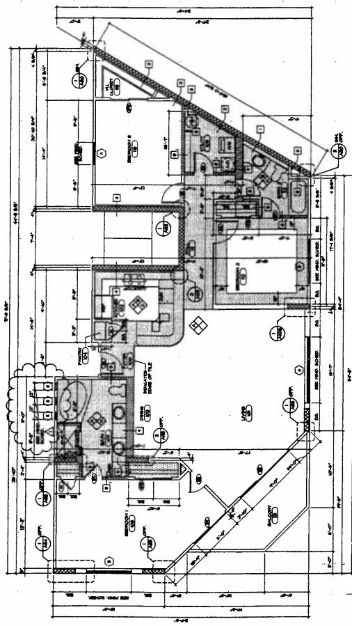
UNIT 'D' FLOOR PLAN
