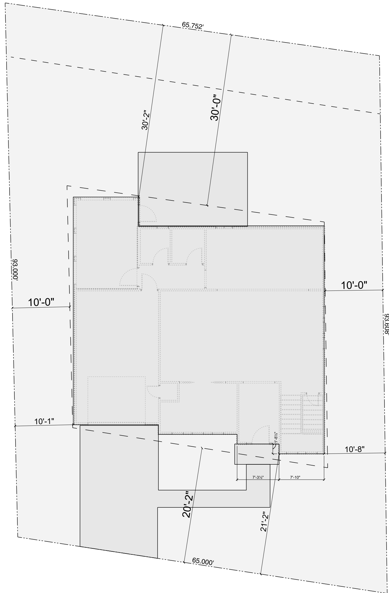
Plot Plan SCALE: 1" = 10'-0"
