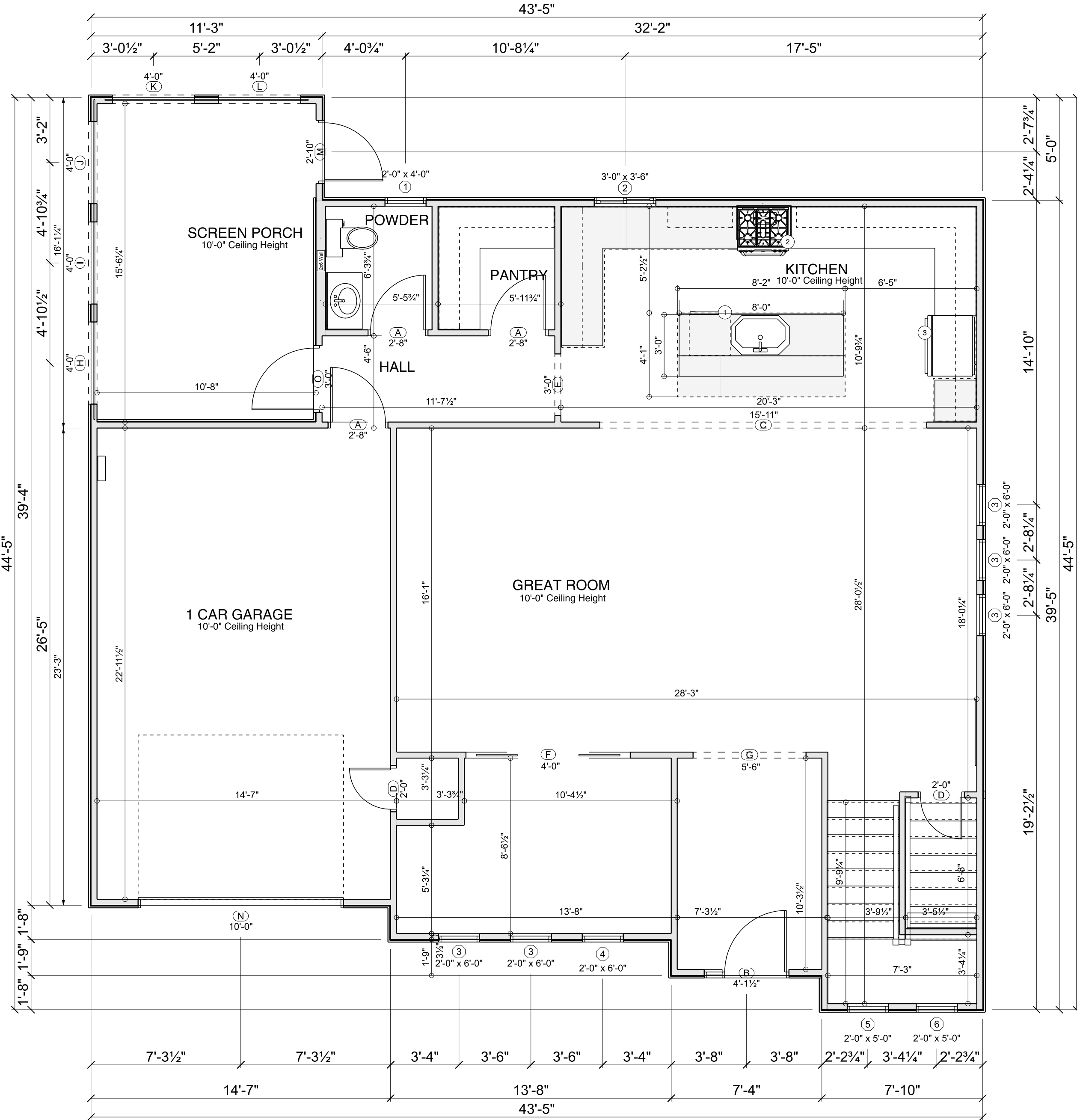
Main Floor SCALE: 1/4" = 1'-0"
