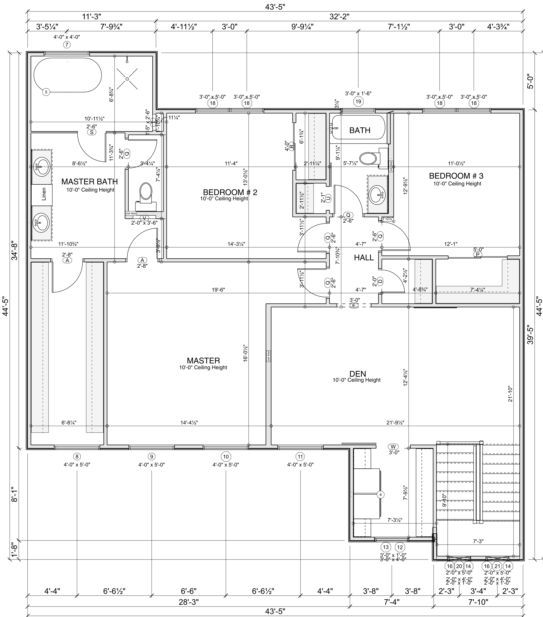
2nd Floor SCALE: 1/4" = 1'-0"
